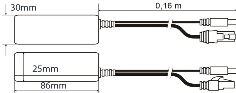
Fig. 1. The mechanical view.
