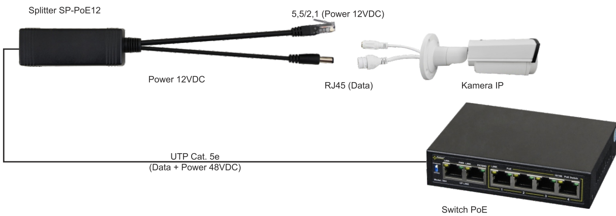
Fig. 2. Example of connection with PoE switch.
