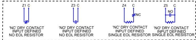
DRY (No EOL Resistor)
