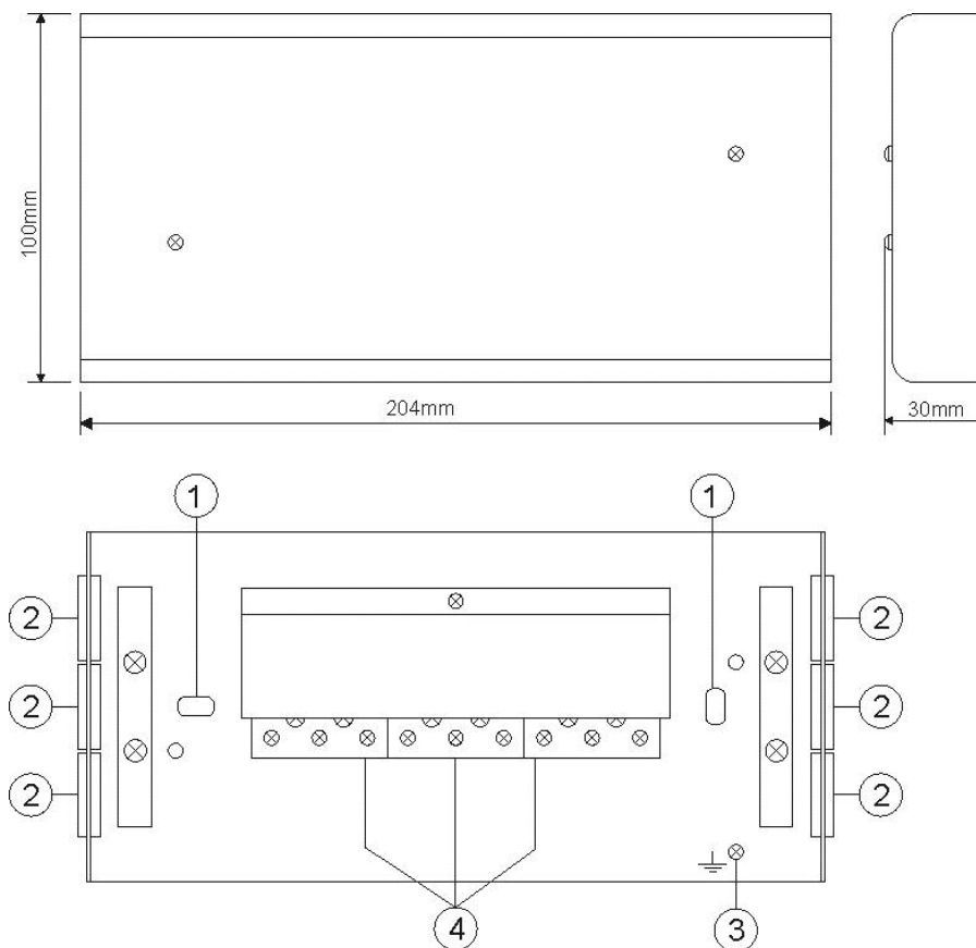
Fig.1. The junction box.
